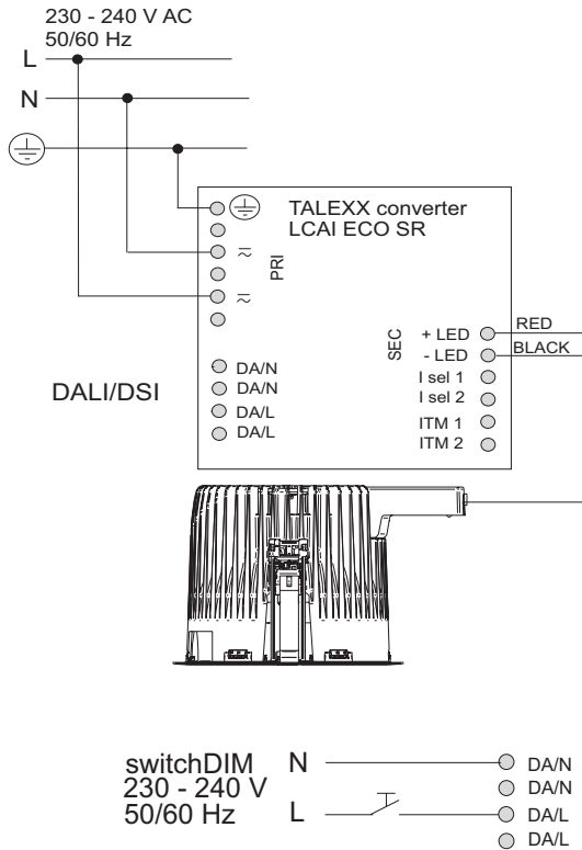
Kopplingschema DALI/SwitchDIM 1100 lm. Wiring diagram DALI/SwitchDIM 1100 lm.
